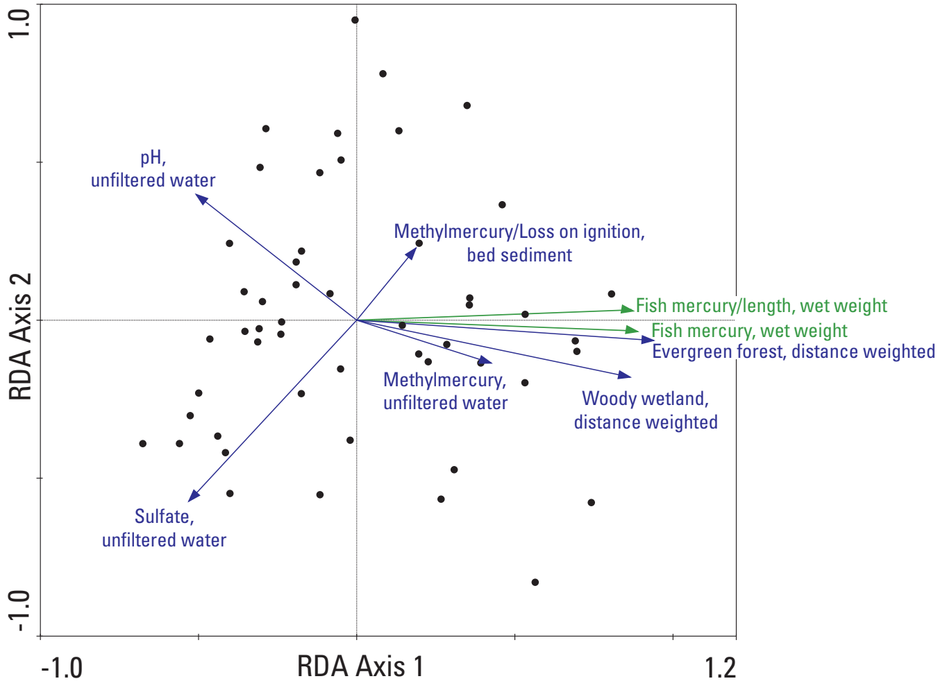
Figure 20. Redundancy Analysis (RDA) showing relative importance of selected environmental characteristics (blue arrows and labels) to concentrations of mercury in largemouth bass (green arrows and labels), 1998–2005. (Arrows extending in the same direction indicate a positive correlation, arrows in opposite directions indicate a negative correlation, and arrows at right angles indicate no correlation; arrow length indicates the relative importance of the variable in the relation.)
