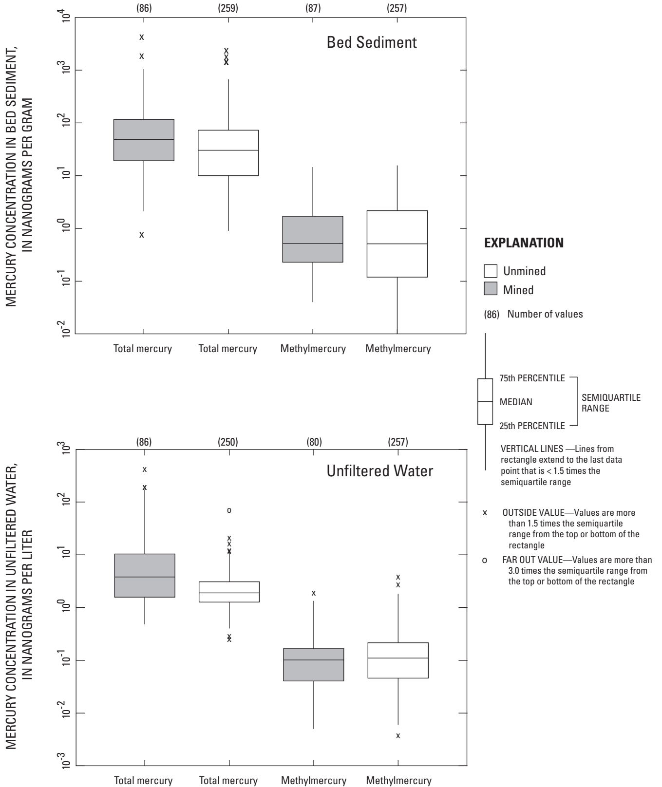
Figure 18. Statistical distributions of mercury concentrations in bed sediment and unfiltered water at stream sites in mined and unmined basins, 1998–2005.
